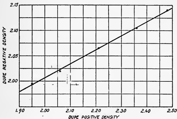
FIG. 6. Combinations of dupe positive and dupe negative which give the same print optima as the original negative.
